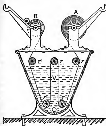
FIG. 3.—Dye-jigger.
