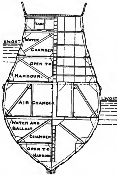
FIG. 25.—Ship Caisson. Scale 1/200.
