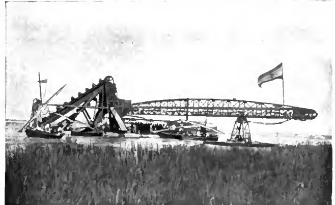
FIG. 6.—Light-draught dredger, with delivery apparatus working round an arc of 210°, by Hunter & English.
