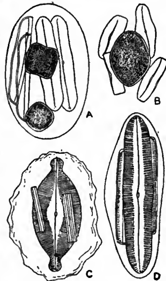
FIG. 6.—Formation of Auxospores.
