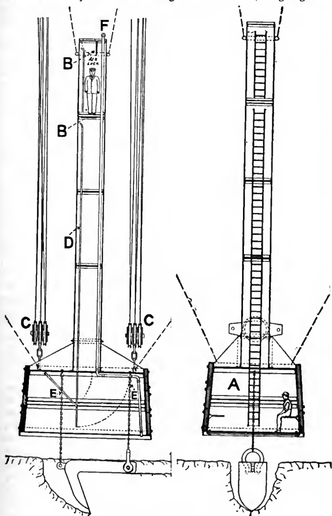
Fig. 7.—Air-lock Diving Bell.
