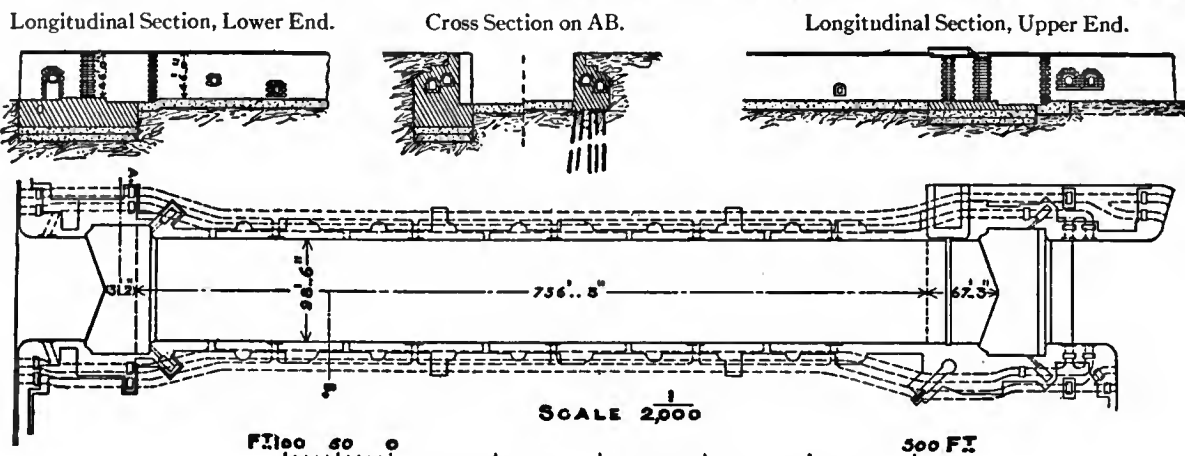
FIG. 20.—Florida Lock, Havre Docks, Sections and Plan.
