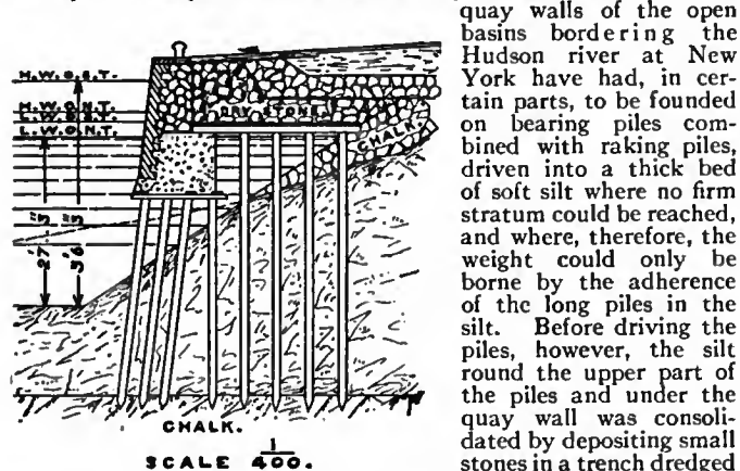
FIG. 17.—Rouen Quay Wall.
