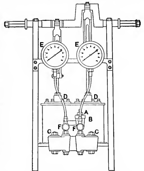
FIG. 1.—Pump out of chest. Two-cylinder, Double-acting Air Pump for Two Divers.
