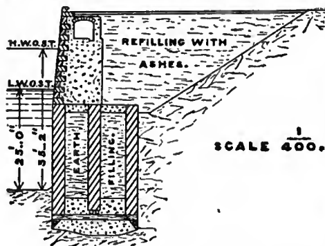
FIG. 16.—Glasgow River Quay Wall.
