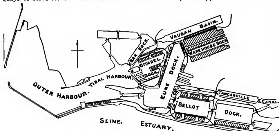
SCALE \frac{1}{30,000} . FIG. 2.—Havre Docks and Outer Harbour.
