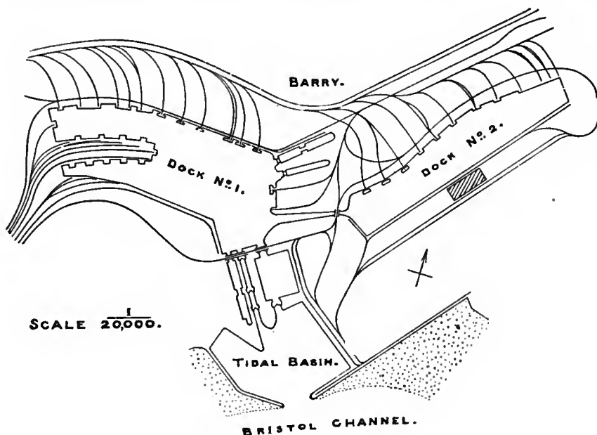
FIG. 8.—Barry Docks.
