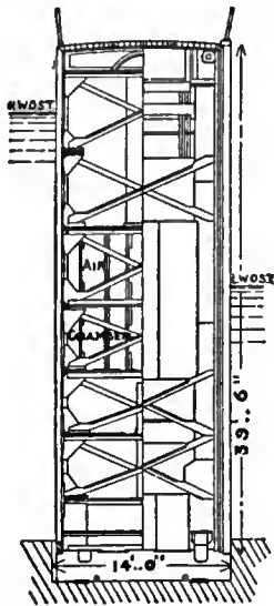
FIG. 24.—Sliding Caisson.
