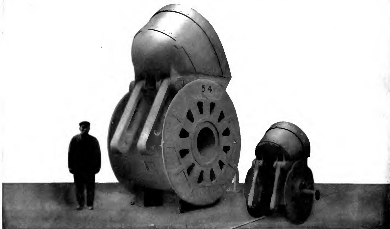
FIG. 11.—BUCKETS OF 5 AND 54 CUBIC FEET CAPACITY COMPARED. The latter, the largest ever made, were for the hopper-dredger "David Dale" (Plate I. fig. 10), built by Lobnitz & Co.
